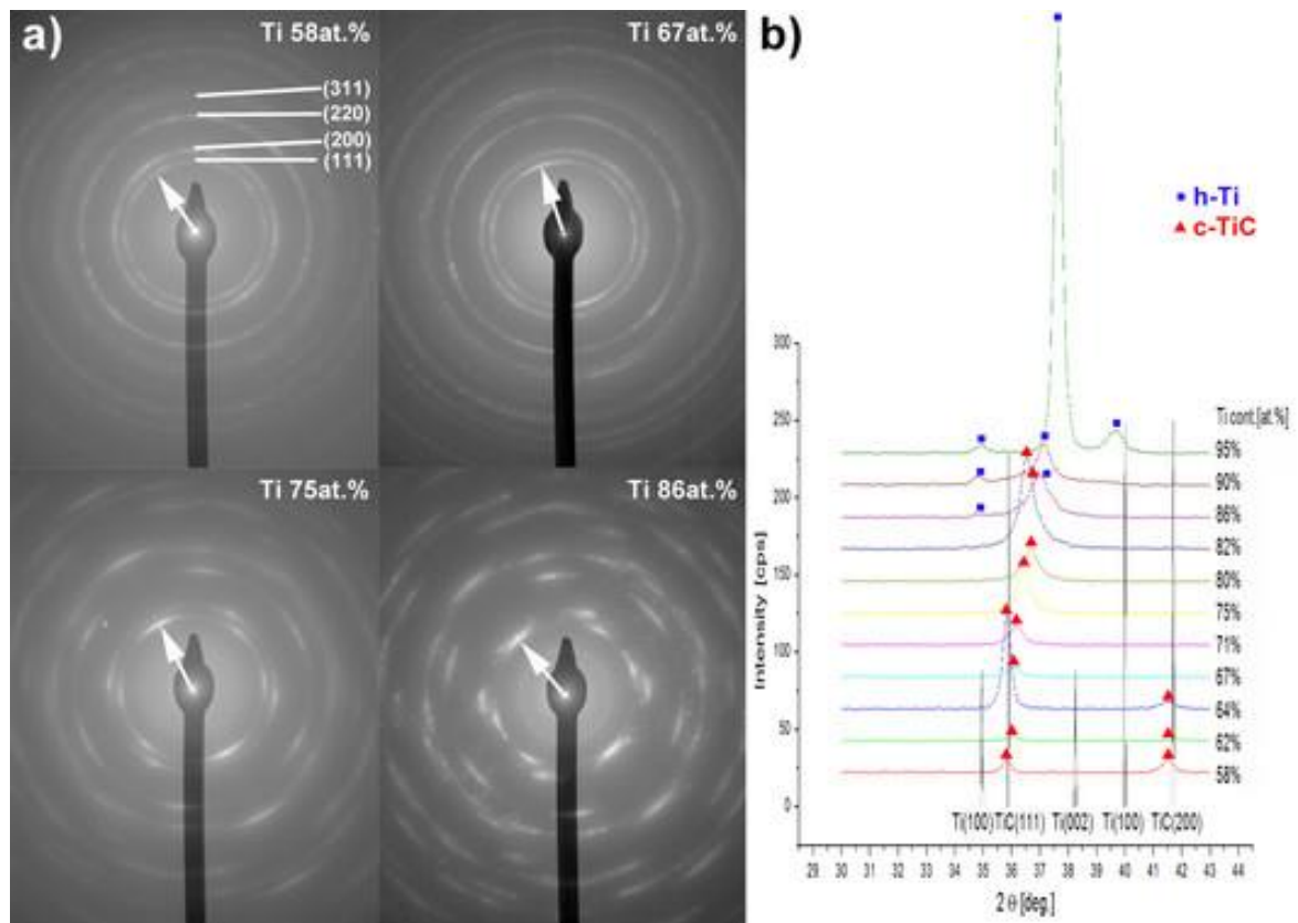
Figure 2. On the left the SAED patterns are shown from the TiC layers containing different amount of Ti. Arrows indicate the direction perpendicular to the surface of the substrate. On the right the XRD patterns of the grown layers.
