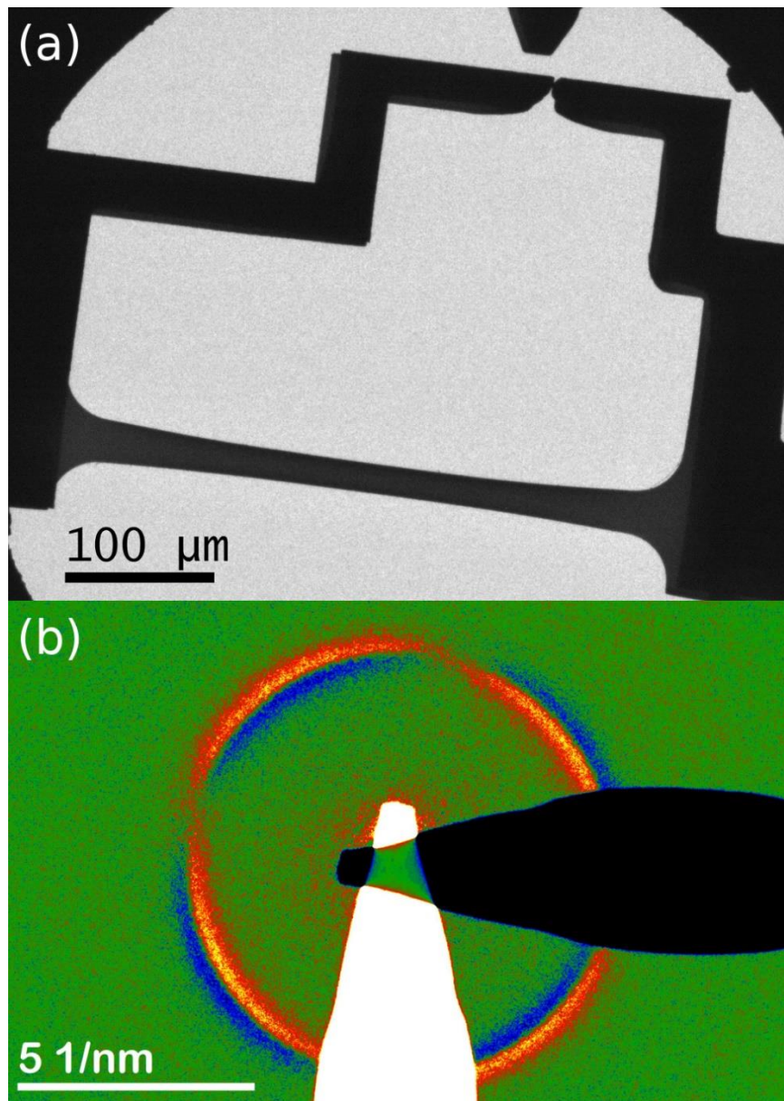
Figure 1. (a) Low magnification image of the amorphous TiAl thin film with the gauges to measure external stress and strain. (b) Color-coded difference image of a highly strained DP and its 90 degree rotated pattern.
